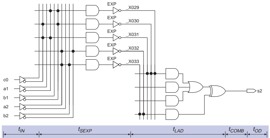
Figure 7. Adder Equations Mapped to MAX 5000 Architecture
